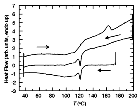
FIG. 8. DSC-cycle of hexagonal 147/260-PF2/6. The linear base-line corrected curve reveals the ill-defined kink at somewhat above 80 °C potentially representing a glass transition (cf. Nothofer [75]). Data show an order-order transition at 155–167 °C and 118–122 °C upon heating and cooling, respectively.
