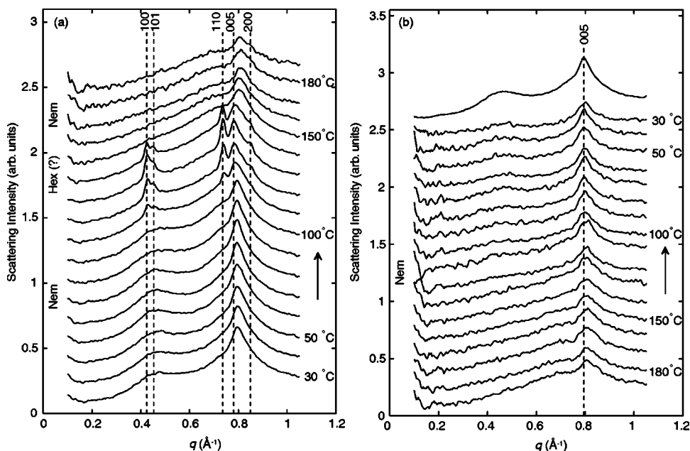
FIG. 13. The powder XRD patterns of 8/15-PF2/6 as a function of temperature during slow (a) heating and (b) cooling (both 0.2\text{ }^{\circ}\text{C/min} ) at intervals of 10^{\circ} . The sample is characteristically nematic with c=39.51\text{ }\text{\AA} but traces of hexagonal phase may appear between 110 and 130\text{ }^{\circ}\text{C} with a=17.06\text{ }\text{\AA} and c=40.18\text{ }\text{\AA} . Note that the scan is not reversible on cooling.
