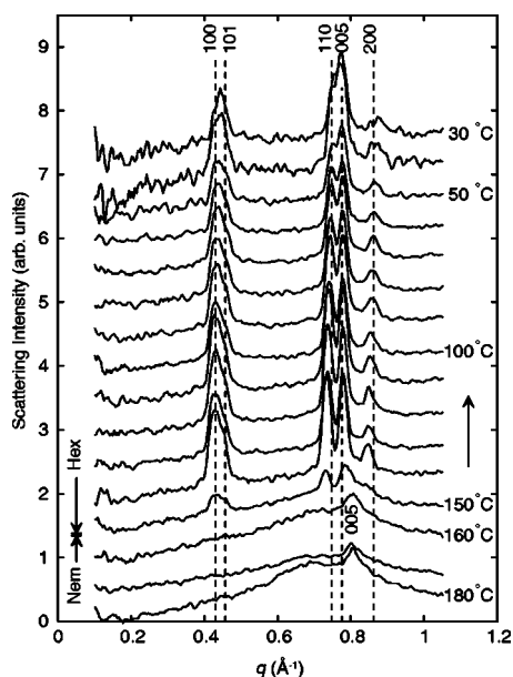
FIG. 12. The powder XRD patterns of 147/260-PF2/6 as a function of temperature during cooling ( 0.2\text{ }^{\circ}\text{C/min} ) at intervals of 10^{\circ} . Note how the hexagonal peaks disappear and the position of 005 reflection changes in the hexagonal-nematic transition at 150\text{ }^{\circ}\text{C} (cf. Fig. 7). The lattice parameters are a=16.82\text{ }\text{\AA} , c=40.46\text{ }\text{\AA} for hexagonal and c\sim 39.5\text{ }\text{\AA} for nematic.
