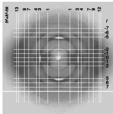
FIG. 15. Two-dimensional fiber XRD patterns of 92/190-PF2/6 at 130°.
